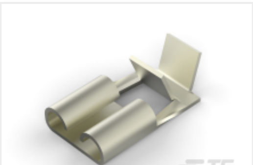
TE 产品编号1217972-2 250 FASTON, FLAG, REC., 18-14 AWG, NPST
