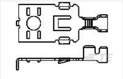
TE 产品编号63496-1 POWER RING TERMINAL TAB 16-10 AWG BR
