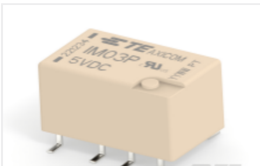
TE 产品编号5-1462039-5 IM03PGR=IM RELAY 140mW 5V
