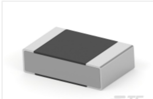
TE 产品编号2176272-7 RU 0805 3K32 0.01% 2PPM 1K RL
