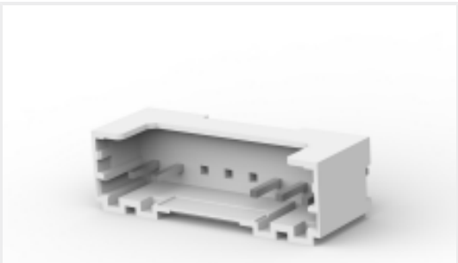
TE 产品编号1971200-1 GIC 2.0 EV 5/8P HEADER ASSEMBLY
