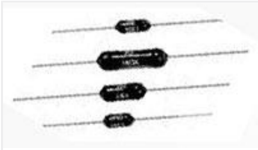
TE 产品编号4-1879639-8 H4P 95R3 0.5% 50PPM
