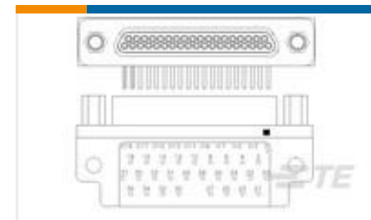
TE 产品编号1532255-4 M83513/10-F01NP = MCKS-N1-P-37PRT1
