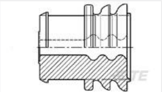
TE 产品编号206425-1 17-3 RECPT. REV SEX
