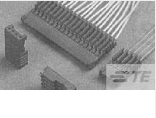
TE 产品编号1-281786-2 PLUG HE14 IDC 180 12 P AWG 28-26
