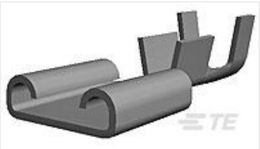
TE 产品编号5-160506-2 250 FASTON REC 20-16 AWG TPBR
