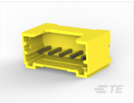
TE 产品编号3-1971032-5 5POS HEADER ASSEMBLY FOR GIC 2.0 EV
