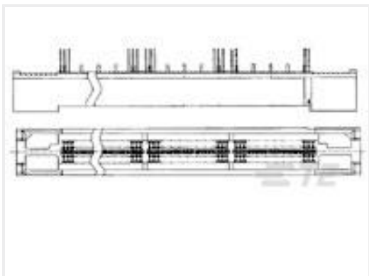
TE 产品编号767044-4 MICTOR,R/A,RECPT,,062,152,ASY
