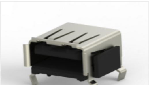
TE 产品编号1674459-4 Std USB Type A, R/A,T/H, Natural, HighDur
