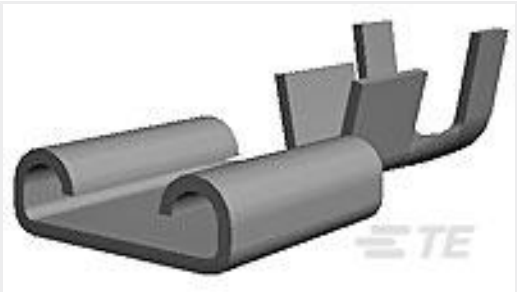
TE 产品编号170180-2 205 FASTON, REC., 18-14 AWG, TPBR
