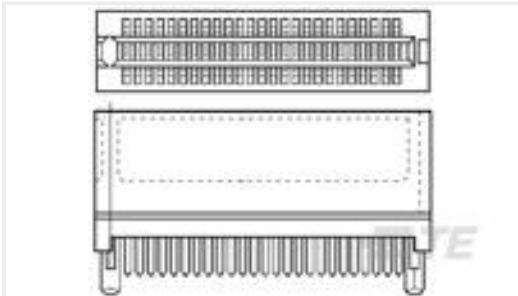
TE 产品编号1658895-2 1SFP 2X6 CAGE & LIGHT PIPE KIT
