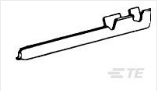
TE 产品编号62358-1 PIN .080 (2.03 MM) 24-20 AWG TPBR
