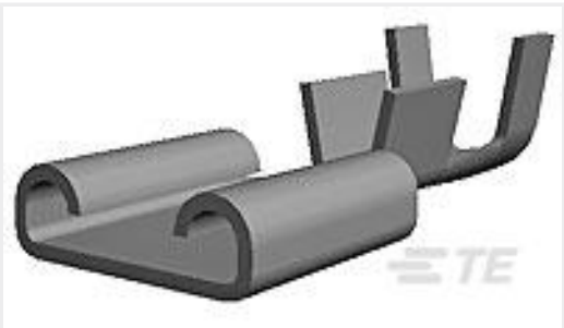
TE 产品编号41774 250 FASTON REC 18-14 AWG TPBZ
