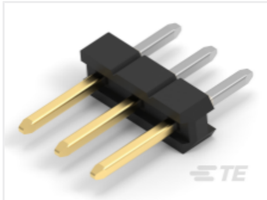
TE 产品编号2355184-4 4P,2MM,BRK HDR,SRVT,2.8,0.76AU,TB W/CAP
