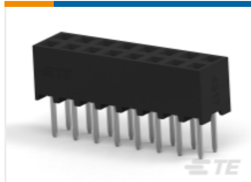
TE 产品编号1-2314824-6 16P,2MM,B-B,REC,DRVT,2.7,0.1AU,TB, W/CAP
