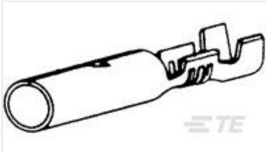
TE 产品编号42531-2 SHUR PLUG 180 RECEPTACLE 20-16 AWG TPBR
