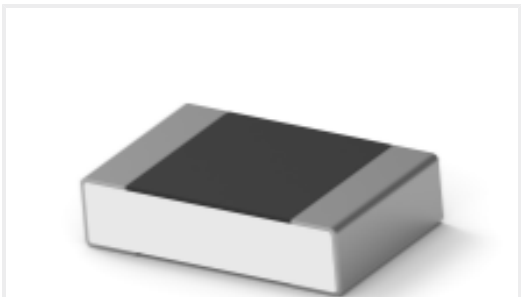
TE 产品编号3-2176379-0 RQ 0805 215R 0.1% 10PPM 5K RL
