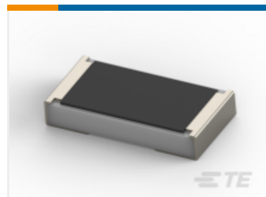
TE 产品编号2176469-4 TLRP 2010 2.0W R050 1% 75PPM 4K RL
