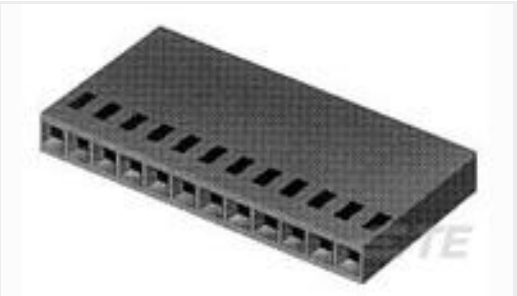
TE 产品编号3-87499-7 20 MODIV HSG SR MRKD .100CL
