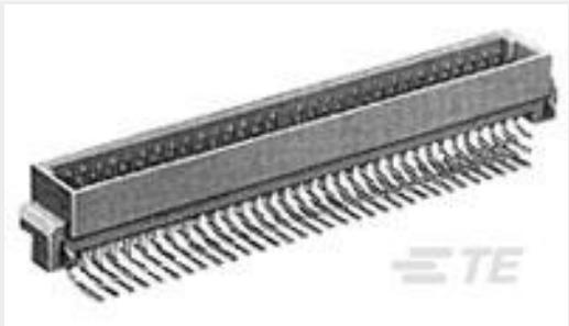
TE 产品编号5650951-5 ASSY, PIN, EUROCARD, TYPE C, LEAD-PB, SCW/QC
