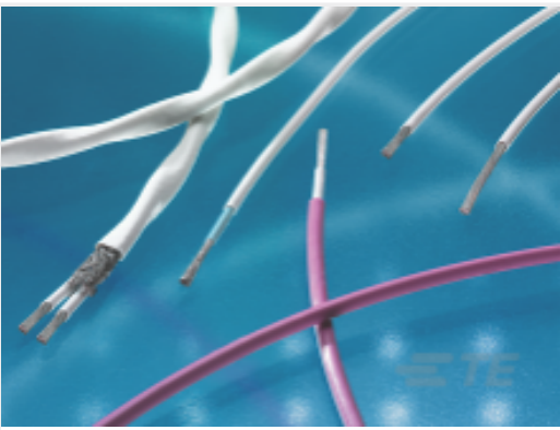
TE 产品编号CAT-55PC-S-TP-8-20 Single Core Twisted Pair Cable: Silver Coated, 8-20 AWG
