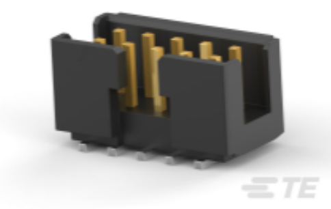
TE 产品编号1-2373376-0 10P,2MM,SHRD HDR,DRVVT,SMD,0.1 AU,TB
