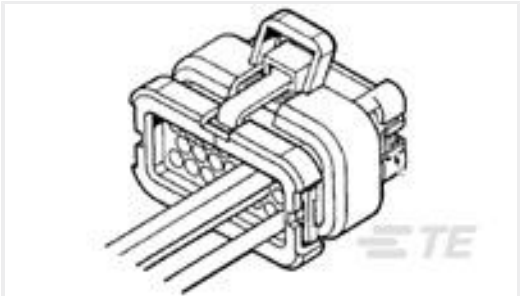
TE 产品编号770680-1 23POS, AMPSEAL, SOC HSG ASSY, SLD, COD 1
