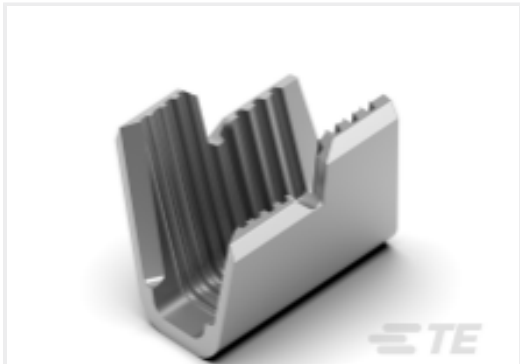
TE 产品编号2238236-1 SPLICE, AMPLIVAR, PIGTAIL, 2D, 600-7000
