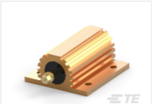
TE 产品编号2-2176732-8 HSC150S 18R 5% Screw Terminal
