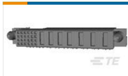
TE 产品编号6450572-1 MBXL R/A RCPT 3ACP+4P+24S
