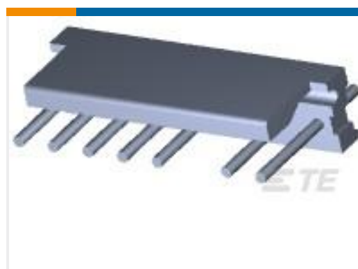
TE 产品编号641938-6 08P MTA156 HDR W/O#3 .045 RD
