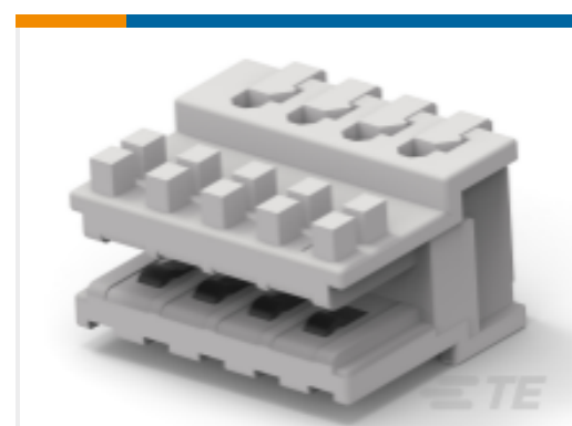
TE 产品编号2311500-4 DUOPLUG STANDARD, FEMALE CONN.
