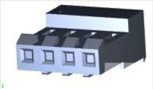
TE 产品编号3-644860-4 04P MTA156 CONN ASSY 18AWG LF
