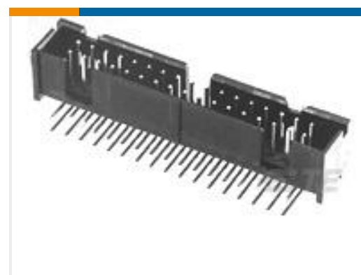
TE 产品编号5103311-7 A/L LOW PRO HDR 34P RA BLACK
