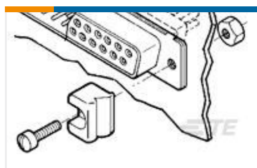
TE 产品编号745286-2 LATCHING BLOCK
