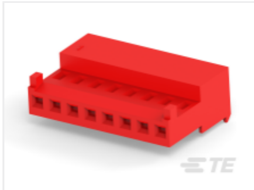
TE 产品编号 CAT-104MTA-NGPMR Nylon Gold Plated Receptacle: 2.54 mm, with Mating Alignment, MTA 100
