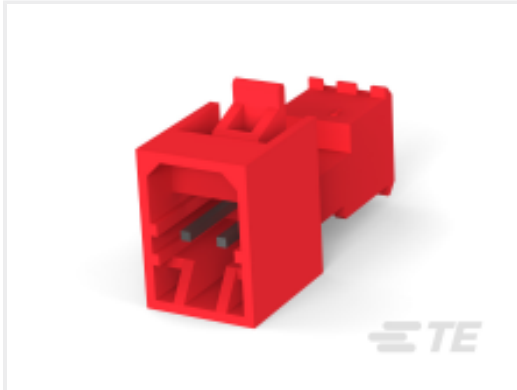
TE 产品编号 CAT-104MTA-NTPMP MTA Plug: Nylon, Tin Plated, 2.54 mm, with Mating Alignment
