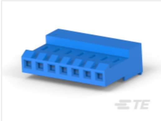
TE 产品编号 3-640430-7 07P MTA156 CONN ASSY 26AWG BLU
