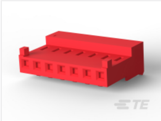
TE 产品编号 3-644463-7 07P MTA156 CONN ASSY 22AWG RED
