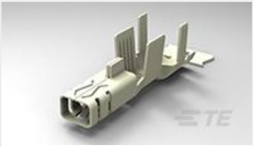
TE 产品编号1742543-1 250 FASTON,FLAG,REC.,18-12 AWG, NPST
