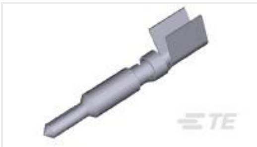
TE 产品编号770246-3 UMNL II PIN PTPPHBZ LP 12-10
