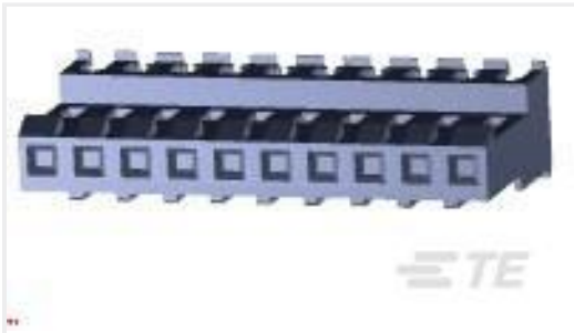
TE 产品编号4-640601-0 10P MTA156 CONN ASSY 22AWG LF
