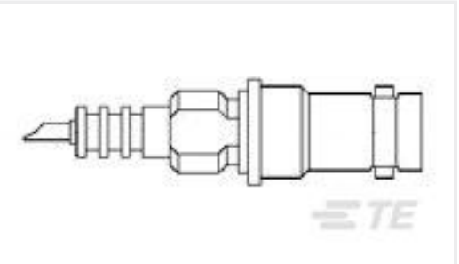
TE 产品编号5225059-3 SHV Jack Str Bulkhead Crimp RG-59, RG-62
