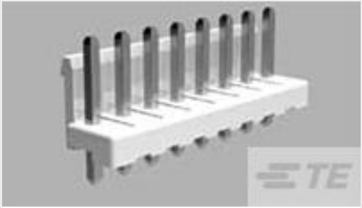
TE 产品编号1-1123723-9 3.96 EP HDR ASSY 9P(NATURAL)
