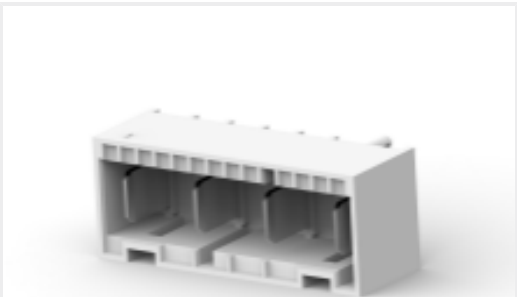
TE 产品编号1-2232511-7 7P, RAST 5 TAB HEADER, THV
