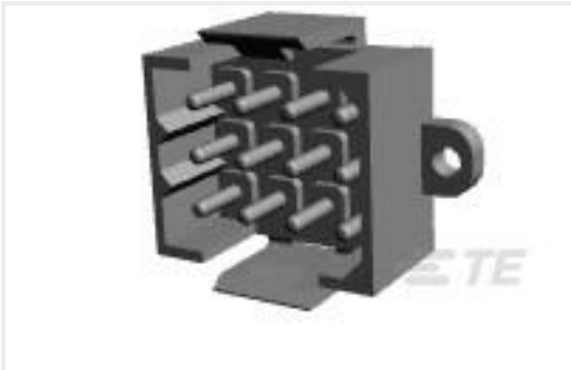
TE 产品编号207120-8 METRIMATE PIN HEADER ASSY,12P
