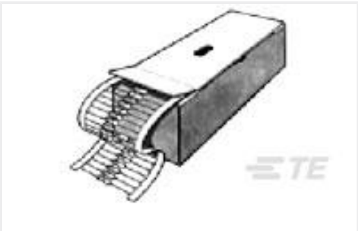
TE 产品编号2176081-9 EP 1W (S) 220R 5%
