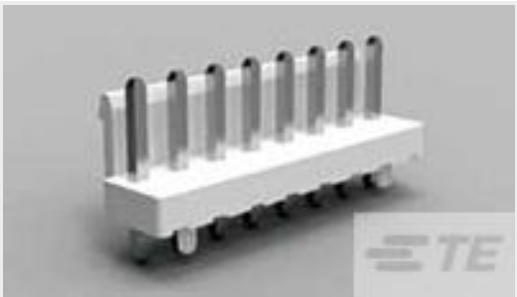
TE 产品编号1744429-9 3.96 EP HDR ASSY 9P W/PEGS, GW
