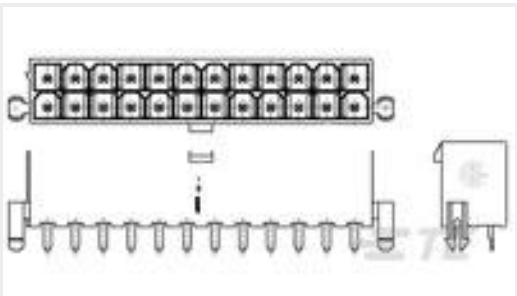
TE 产品编号1-2029265-4 14P VAL-U-LOK VRTHDR W/PGS GW
