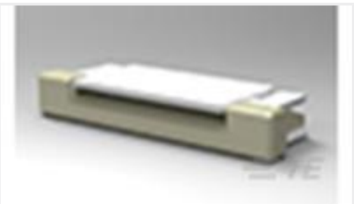
TE 产品编号4-1734839-0 FPC CONN. 0.5MM PITCH T/C,40P
