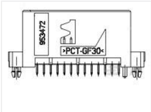
TE 产品编号953472-1 26pos MQS .63 header 180deg THR
