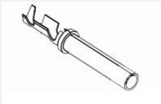
TE 产品编号776492-2 SOC, SF, SIZE 16, 14-18 AWG, NI/SN
