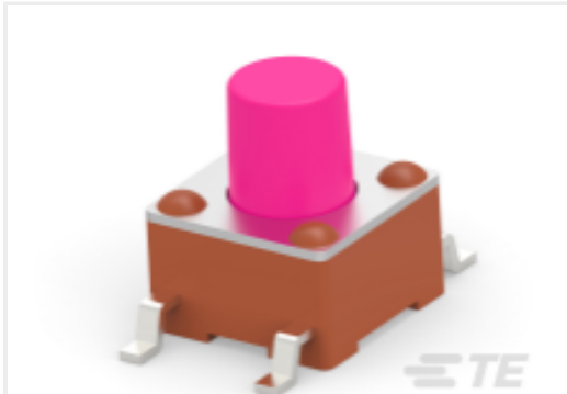
TE 产品编号2-1977223-0 FSM6JSMASTR=6MM TACT SWITCH, SMT 260gf,
