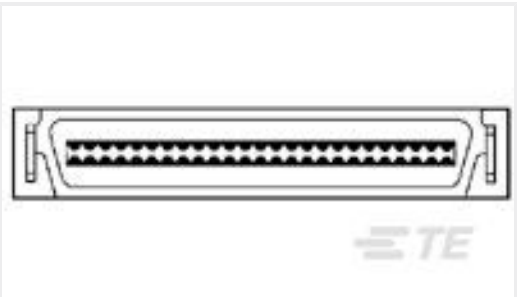
TE 产品编号1-1734101-7 Champ050 series, 50 pos,30u" Au, 3.30 H
