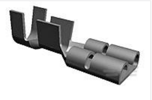
TE 产品编号63306-1 250 FASTON REC 18-14 AWG BR
