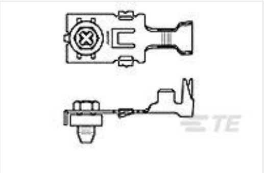
TE 产品编号521843-1 POWER BLOCK ASSEMBLY 16-12 AWG PTPBR
